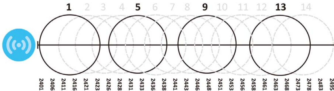
Figure 58 An Alternative Four-Channel Deployment
