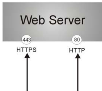
Figure 93 HTTP/HTTPS Implementation
