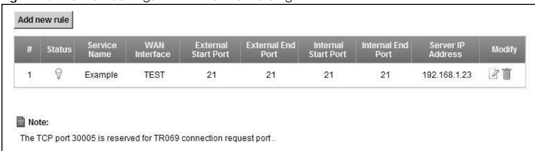
Figure 43 Network Settings > NAT > Port Forwarding
