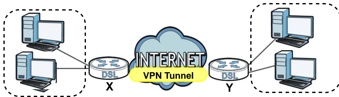
Figure 74 VPN: Example
