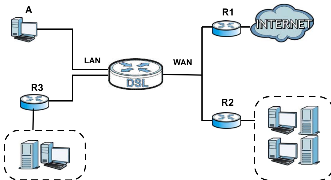
Figure 87 Example of Static Routing Topology
