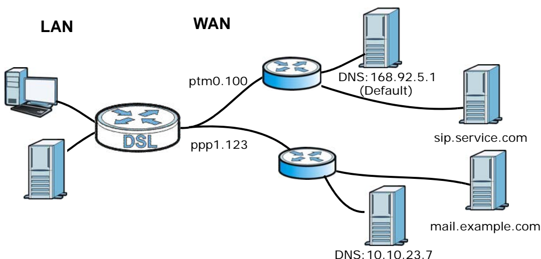
Figure 90 Example of DNS Routing Topology
