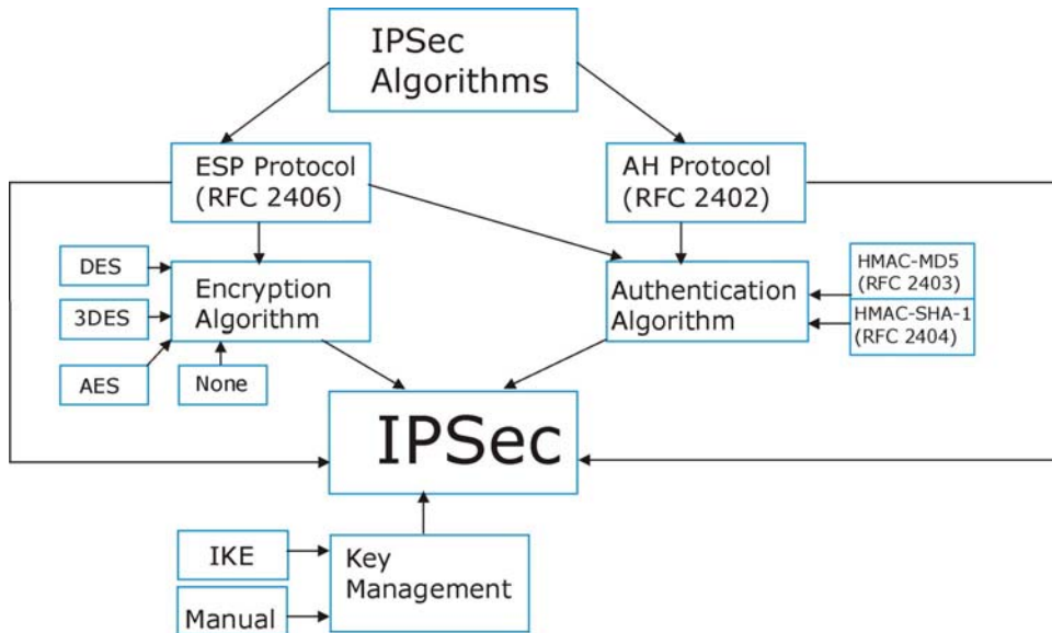
Figure 81 IPsec Architecture
