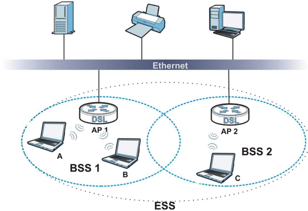
Figure 176 Infrastructure WLAN
