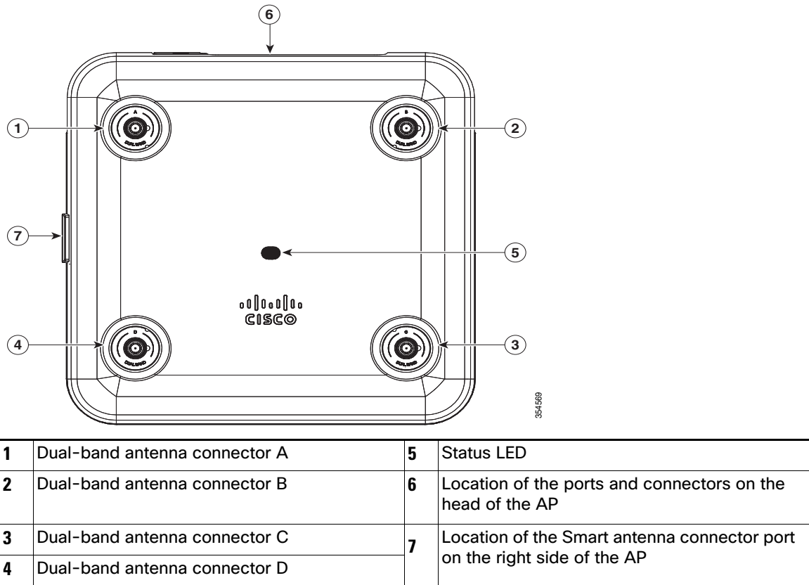
Figure 2 Face of the 2802E Model
