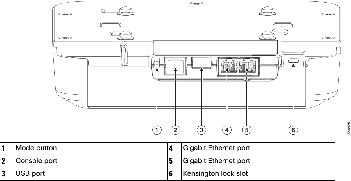
Figure 4 Ports and Connectors on the Head of the 2802I Model
