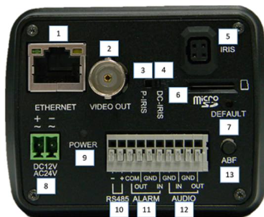
CF-6308 Connector Panel
