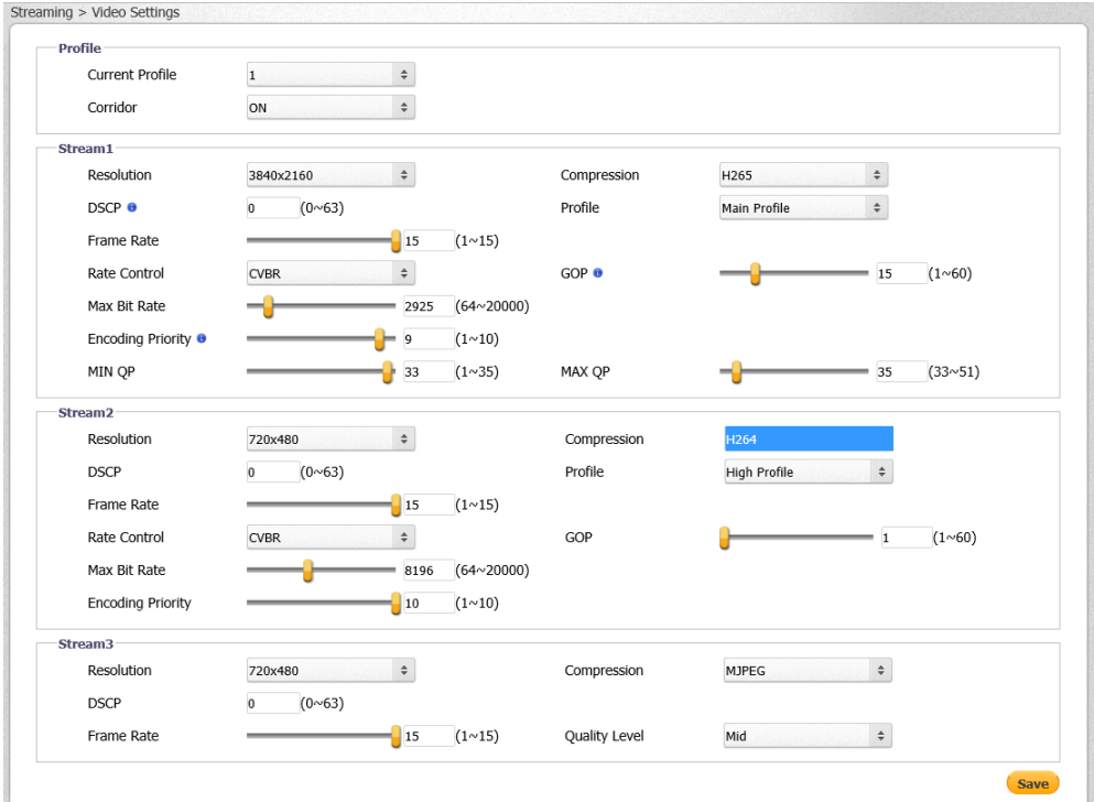
Video Settings Screen
