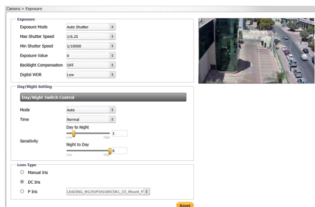
Auto Shutter Exposure Mode Settings
