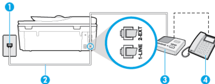
Figure 5-11 Back view of the printer
