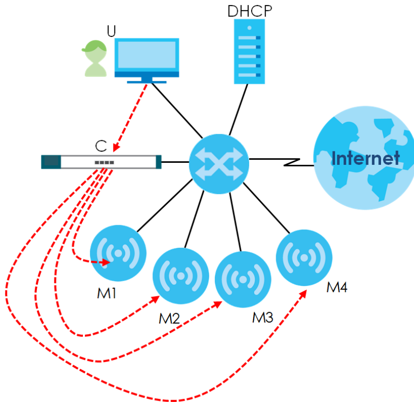
Figure 38 CAPWAP Network Example
