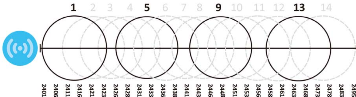
Figure 54 An Alternative Four-Channel Deployment
