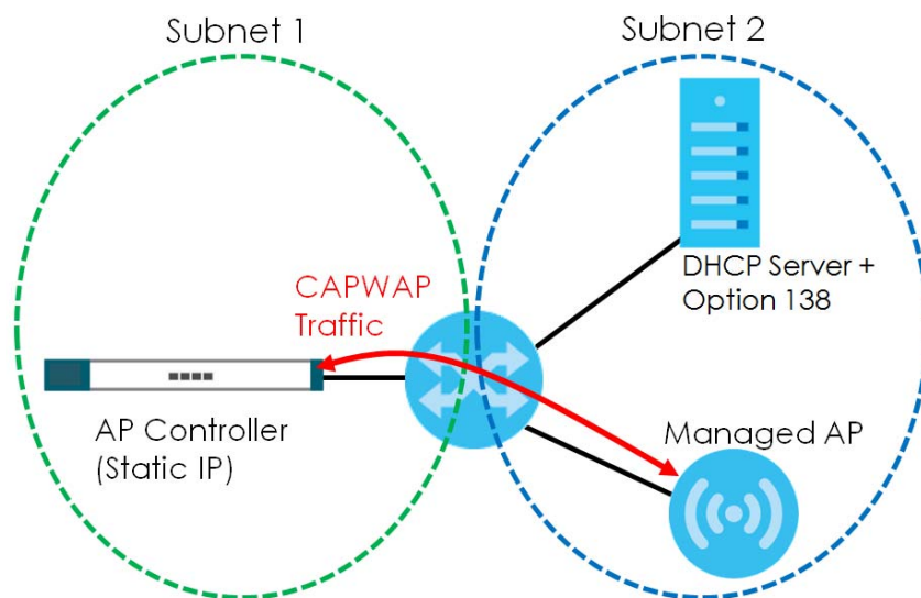
Figure 39 CAPWAP and DHCP Option 138
