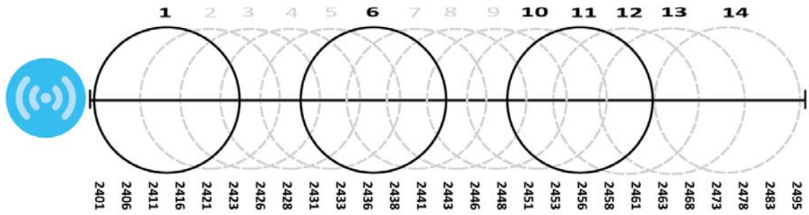
Figure 52 An Example Three-Channel Deployment
