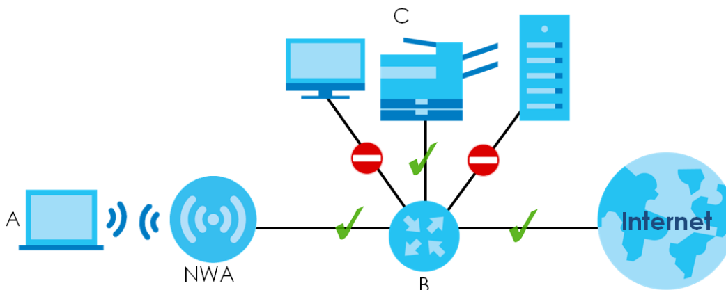
Figure 67 Layer-2 Isolation Application
