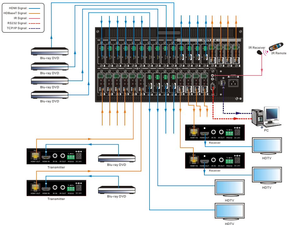
Figure 3- 1 Connection Diagram
