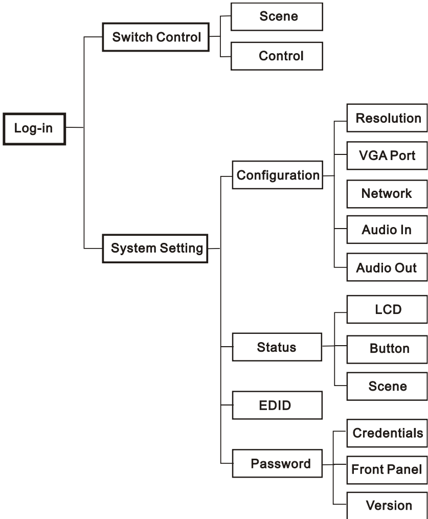
Figure 4- 2 GUI Structure
