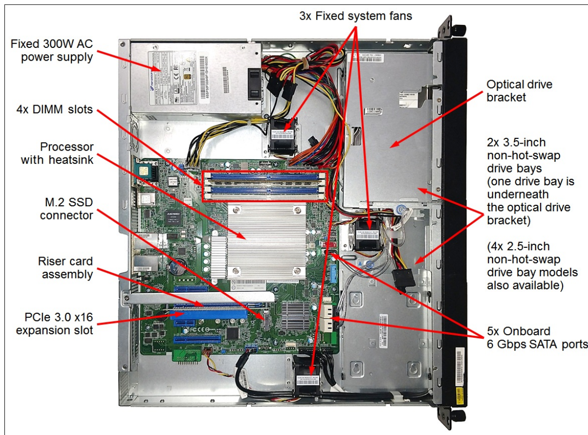
Figure 4. RS160 internal view
