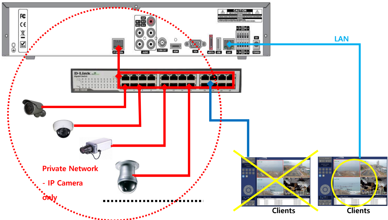
Figure 2.6.1.2. Improper connection of the NS (Non PoE switch).
