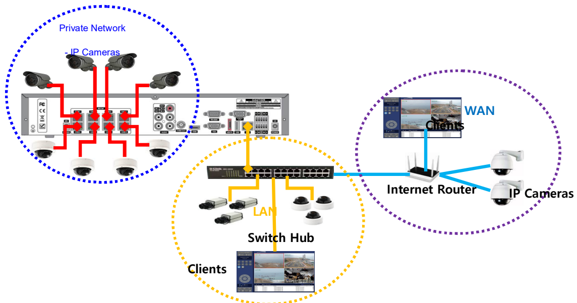
Figure 2.5.1.2 IP Camera Connection Diagram (N16NSP)
