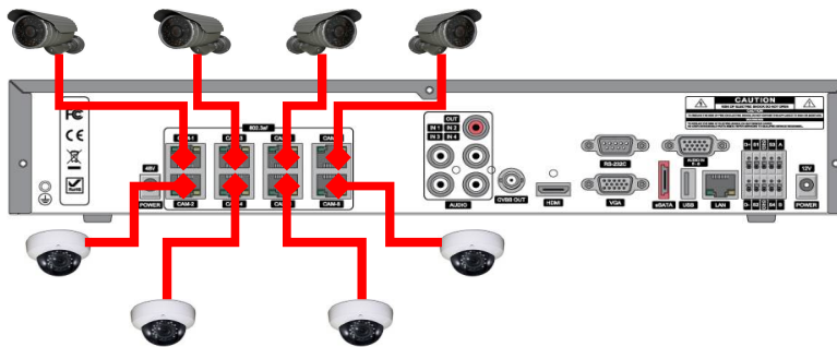
Figure 2.5.1.1 IP Camera Connection Diagram (N8NSP)
