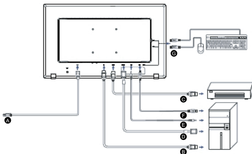
Figure 3 Connecting Cables
