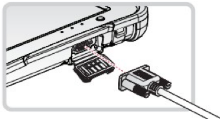
Figure 33. Connect RS-232 Cabling
