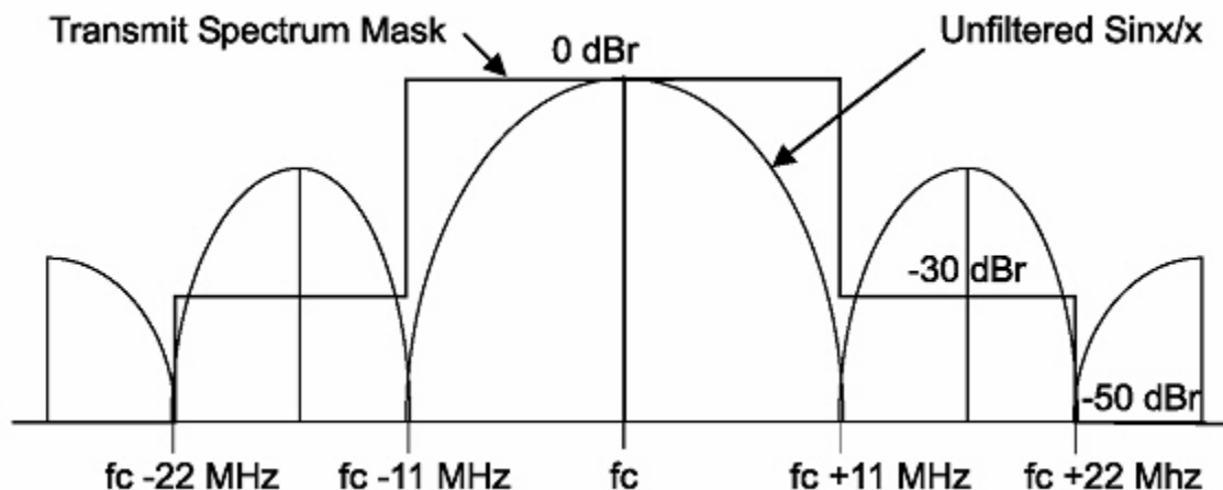
Transmit Spectrum Mask for 802.11b
