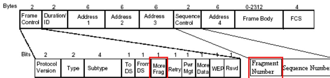
IEEE 802.11 Frame fields for frame fragmentation and defragmentation
