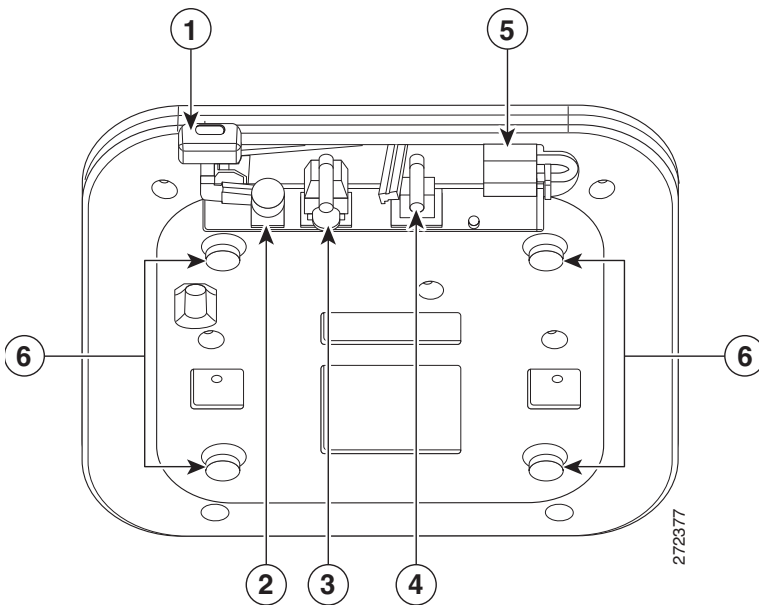
Figure 3 Access Point Ports and Connections (bottom)
