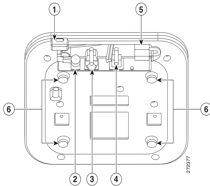
Figure 3 Access Point Ports and Connections (bottom)-AIR3602E and 3602I Models
