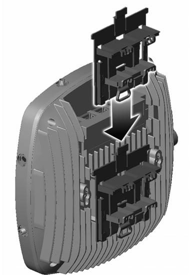
Figure 2-1 Attaching Mount Bracket to the Access Point
