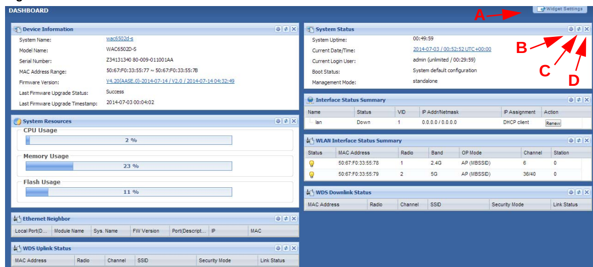
Figure 17 Dashboard
