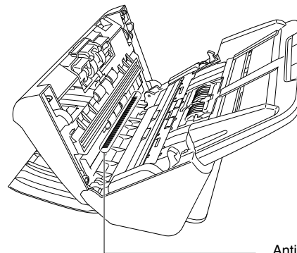
Anti-Static brush
