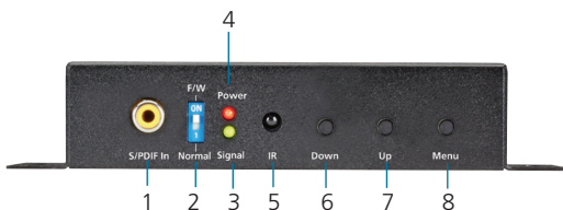
Figure 2-1. Front panel.
