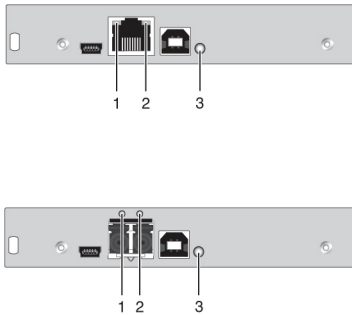
CPU module, rear view
