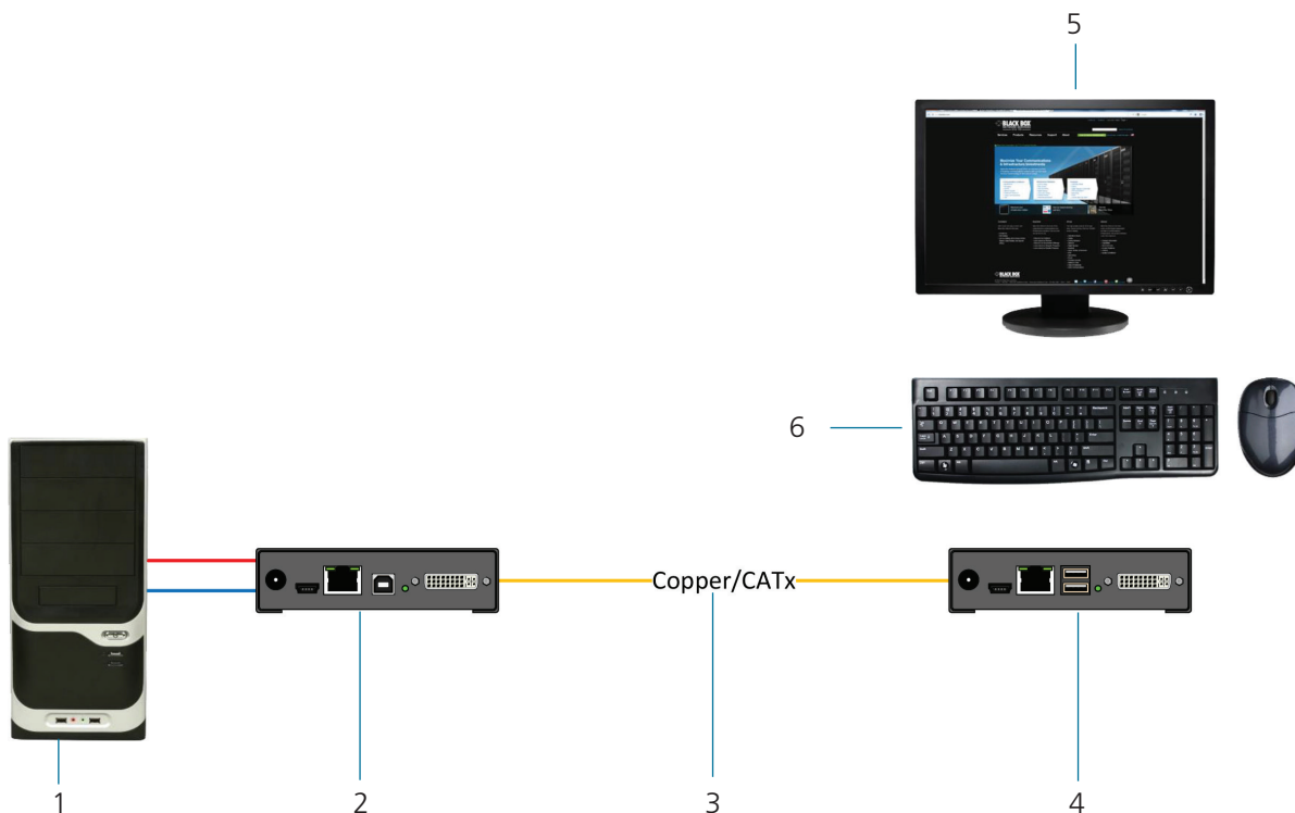
Figure 2-1. System diagram.
