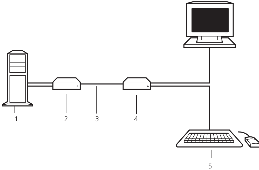
Figure 3-12. DKM Modular Extender (Single-Head).
