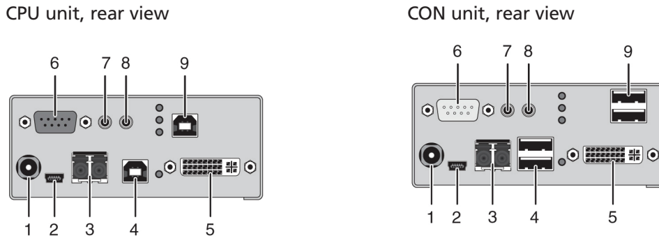
Figure 2-5. ACX1T-12A-SM (CPU unit) and ACX1R-12A-SM (CON unit).
