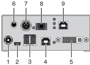
Figure 2-7. ACX1T-12D-SM (CPU unit) and ACX1R-12D-SM (CON unit).
