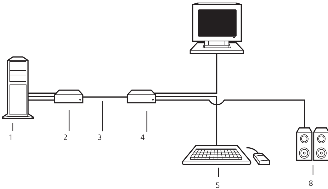
Figure 3-13. DKM Modular Extender (Single-Head with Digital/Analog Audio).
