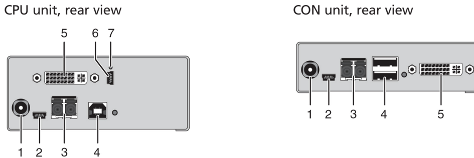
Figure 2-12. ACX1T-11V-SM (CPU unit) and ACX1R-11V-SM (CON unit), rear view.
