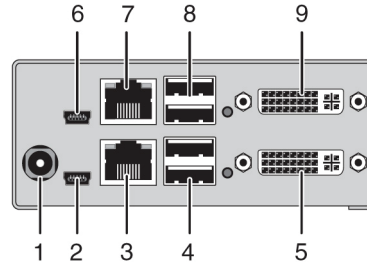
Figure 2-14. ACX1T-22-C (CPU unit) and ACX1R-22-C (CON unit).
