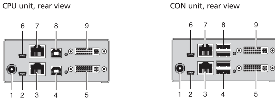
Figure 2-15. ACX1T-22-SM (CPU unit) and ACX1R-22-SM (CON unit).
