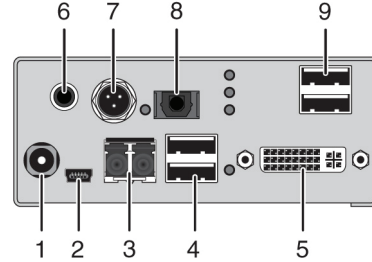
Figure 2-7. ACX1T-12D-SM (CPU unit) and ACX1R-12D-SM (CON unit).
