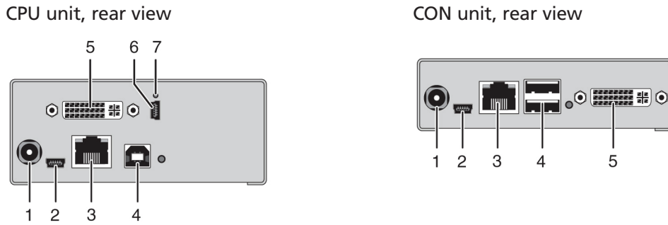
Figure 2-10. ACX1T-11V-C module (CPU unit) and ACX1R-11V-C module (CON unit), rear view.
