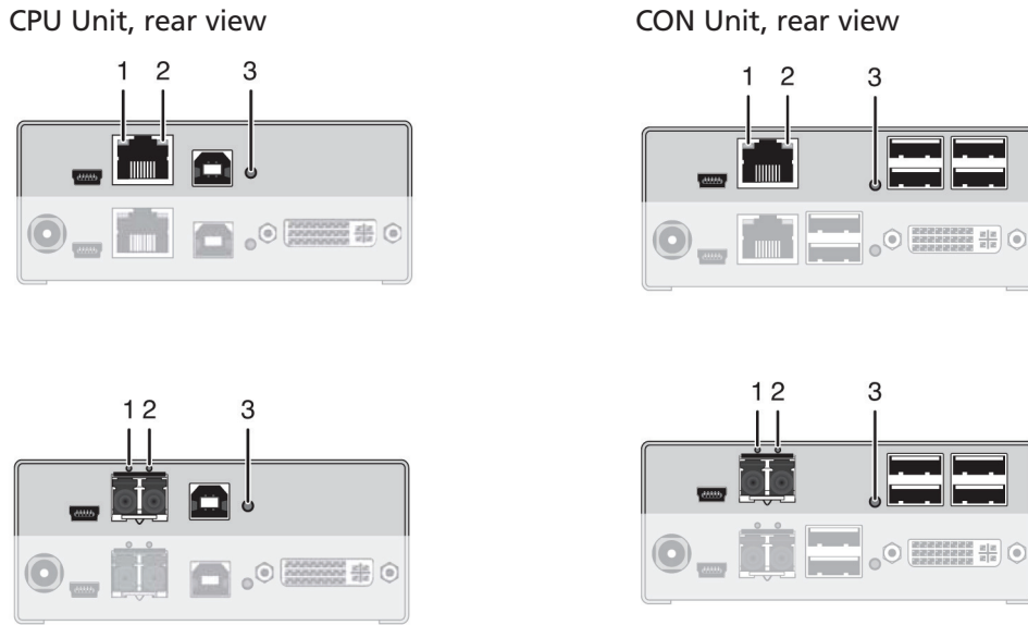
Figure 6-5. USB 2.0 upgrade module.
