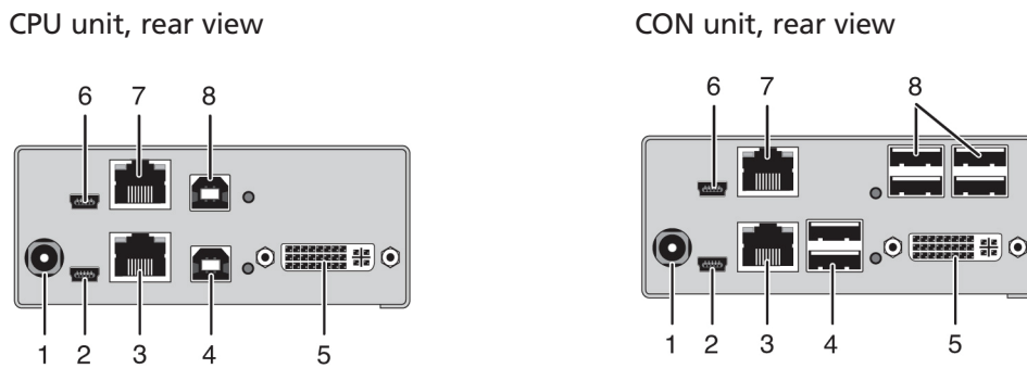
Figure 2-8. ACX1T-13-C (CPU unit) and ACX1R-13-C (CON unit).
