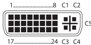
Figure 1-1. DVI-D connector.
