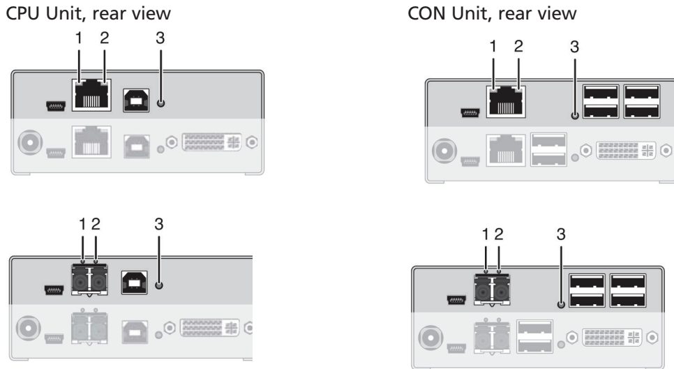
Figure 2-19. Status USB 2.0 (option).
