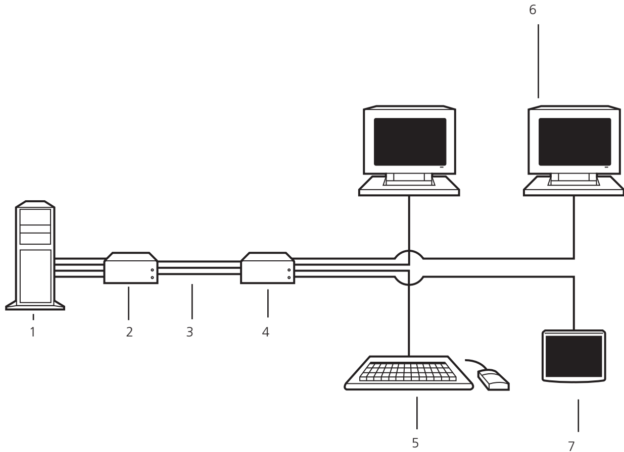
Figure 3-14. DKM Modular Extender (Dual-Head with 4x USB-HID).
