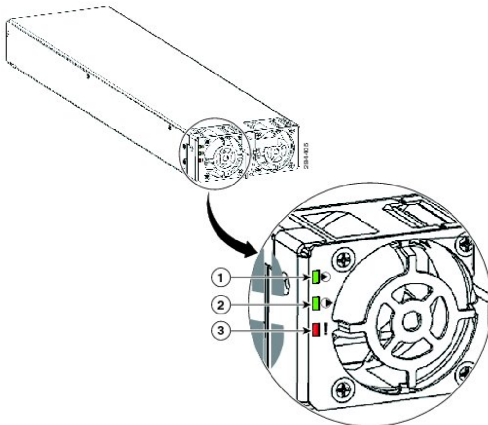
Figure 203: Version 2 Power Module Power Module Status Indicators
