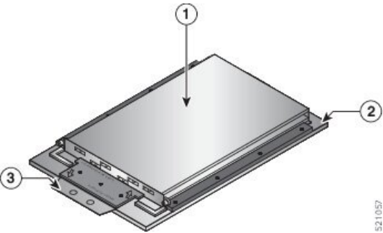
Figure 226: Refixing the Plastic Blocker
