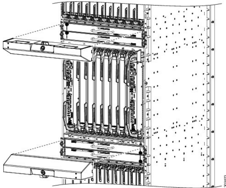
Figure 166: Optional Fan Tray Covers for the Cisco ASR 9922 Router
