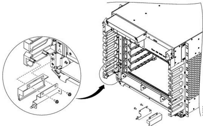
Figure 148: Installing Ball Stud Assemblies on the Cisco ASR 9006 Router (Shown with Version 1 Power System)
