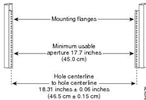
Figure 114: Verifying Equipment Rack Dimensions
