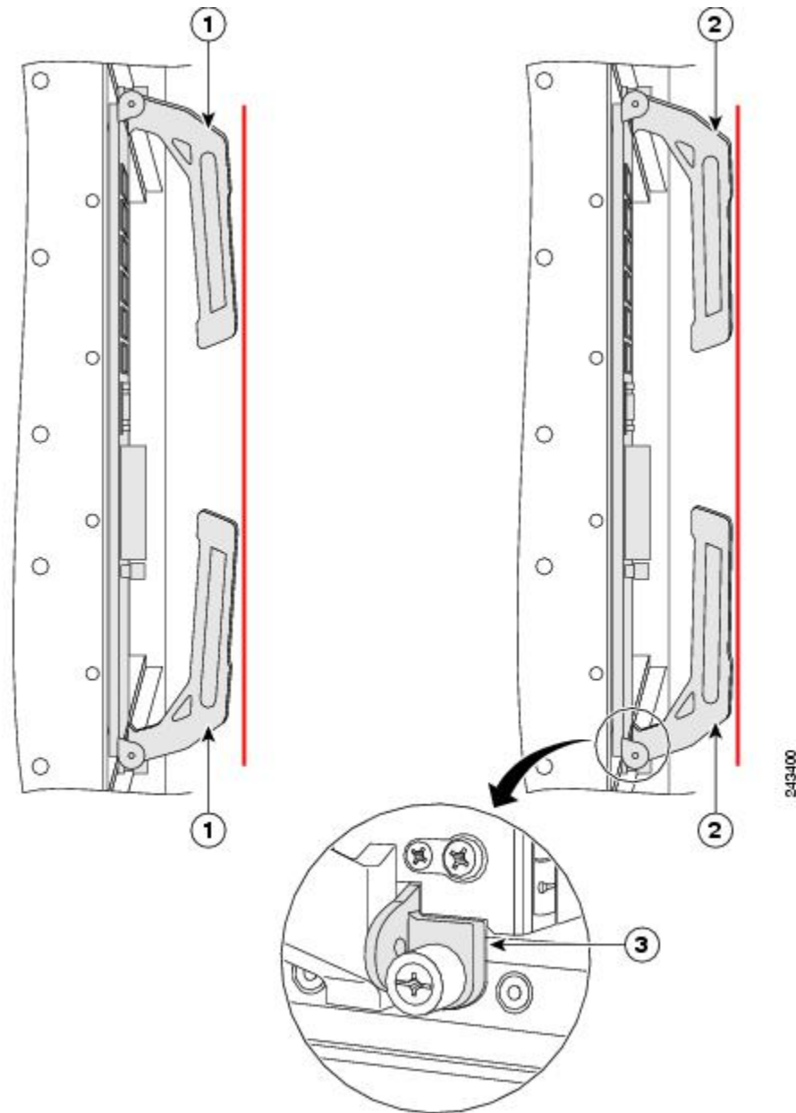
Figure 179: FC Card Ejector Lever Positions During Installation
