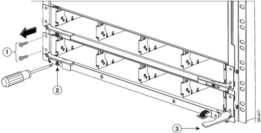
Figure 221: Removing a Power Tray—Version 2 Power Tray (Cisco ASR 9010 Router Shown)
