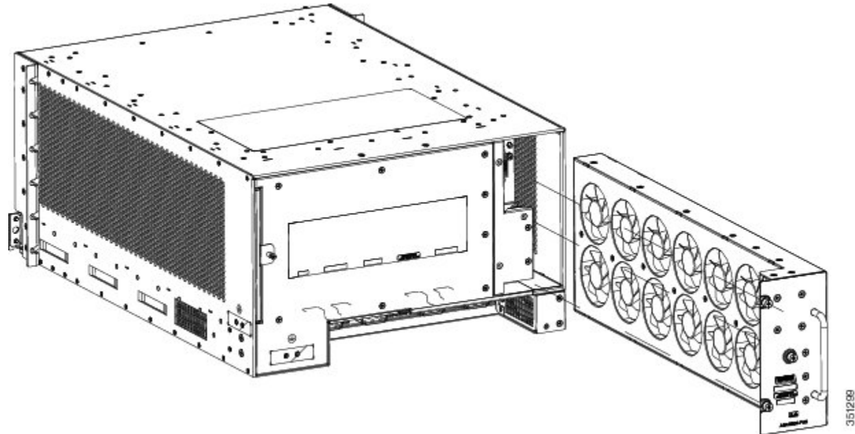
Figure 86: Removing or Installing the Fan Tray on the Cisco ASR 9904 Router Chassis
