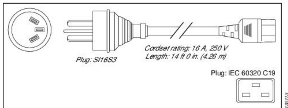
Figure 36: AC Power Cord CAB-AC-2500W-ISRL=
