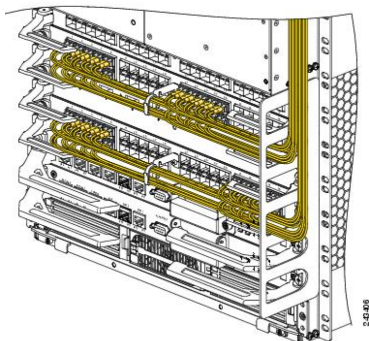
Figure 191: Interface Cable Routing Using the Line Card and Chassis Cable Management Bracket on the Cisco ASR 9904 Router
