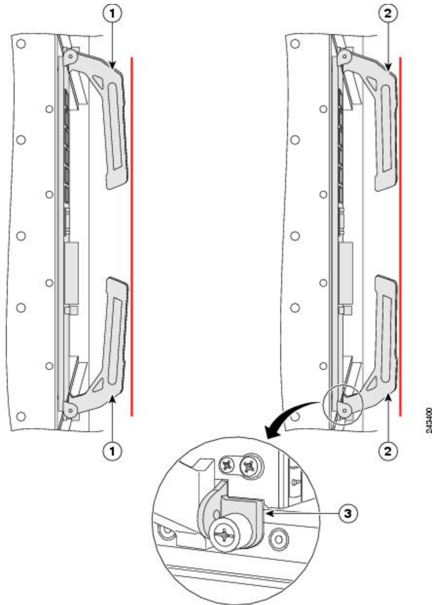
Figure 178: FC Card Ejector Lever Positions During Installation
