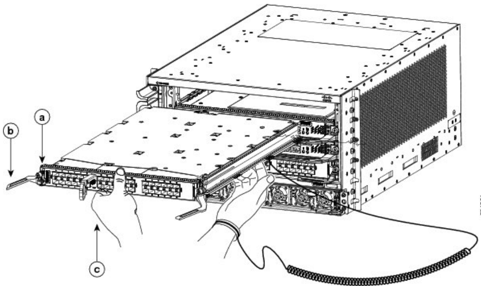
Figure 101: Removing a Line Card from the Cisco ASR 9904 Router Chassis
