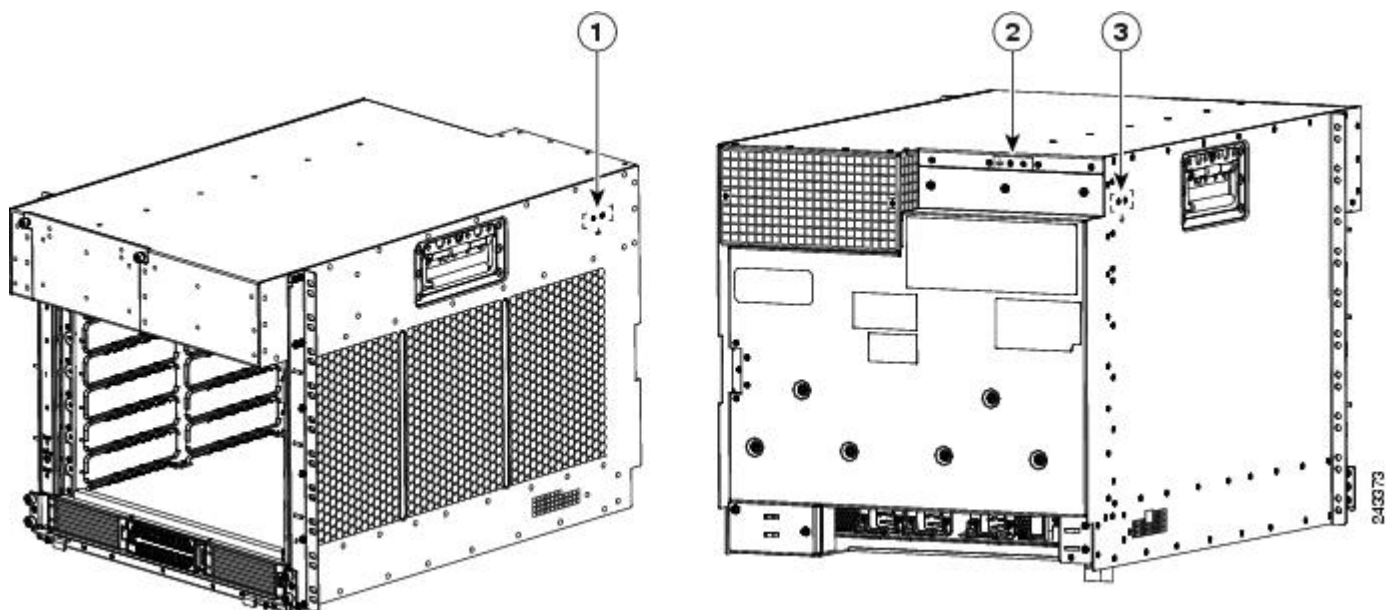
Figure 59: NEBS Bonding and Grounding Point on the Cisco ASR 9006 Router Chassis
