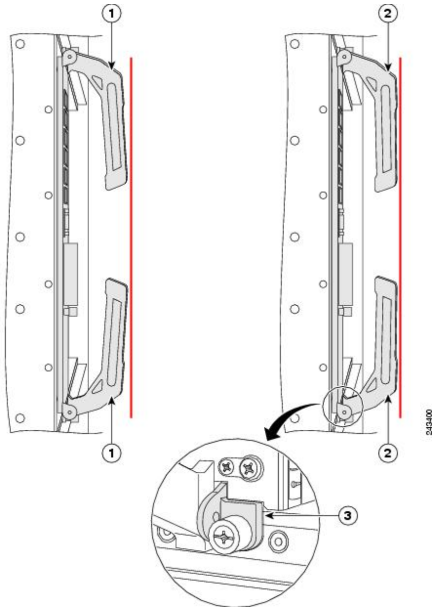
Figure 177: RP Card Ejector Lever Positions During Installation
