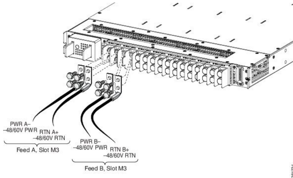
Figure 201: Location of DC Power Switch—Version 2 and Version 3 Power System
