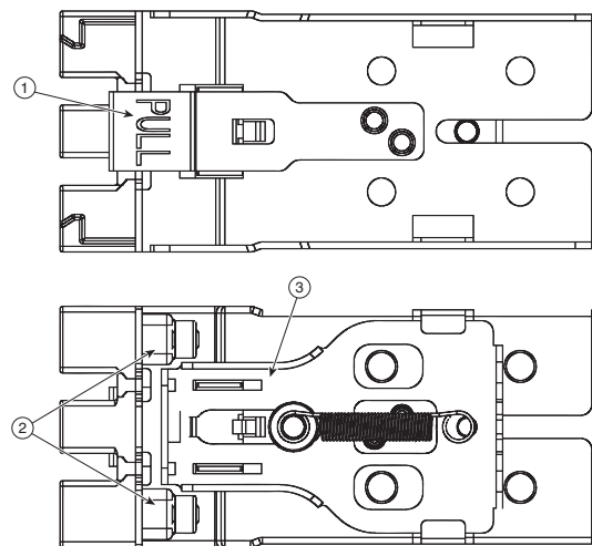
Figure 3-2 Front Securing Latch
