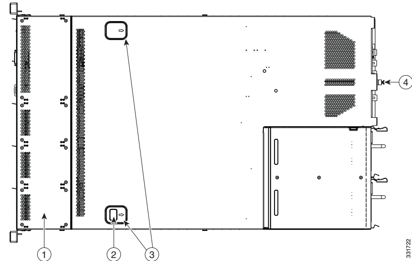
Figure 4-1 Removing the Top Cover: Cisco Connected Safety and Security UCS C220
