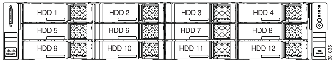
Figure 4-7 Drive Numbering, Large Form-Factor Drives
