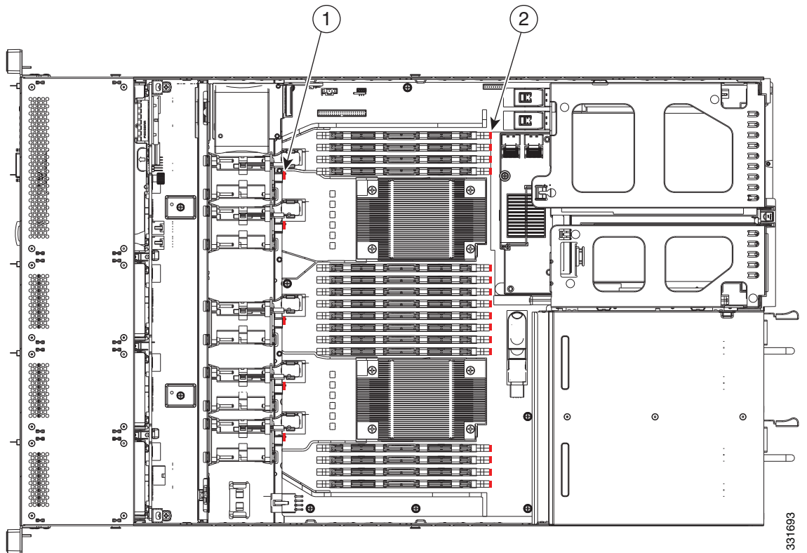
Figure 1-7 Internal Diagnostic LED Locations: Cisco Connected Safety and Security UCS C220
