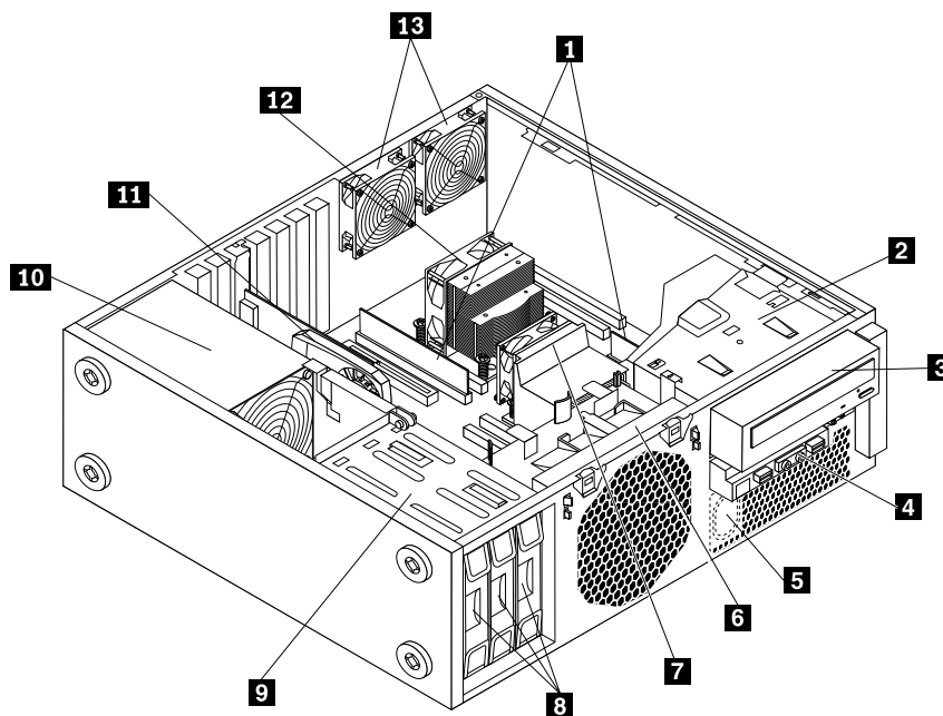
Figure 3. Component locations
