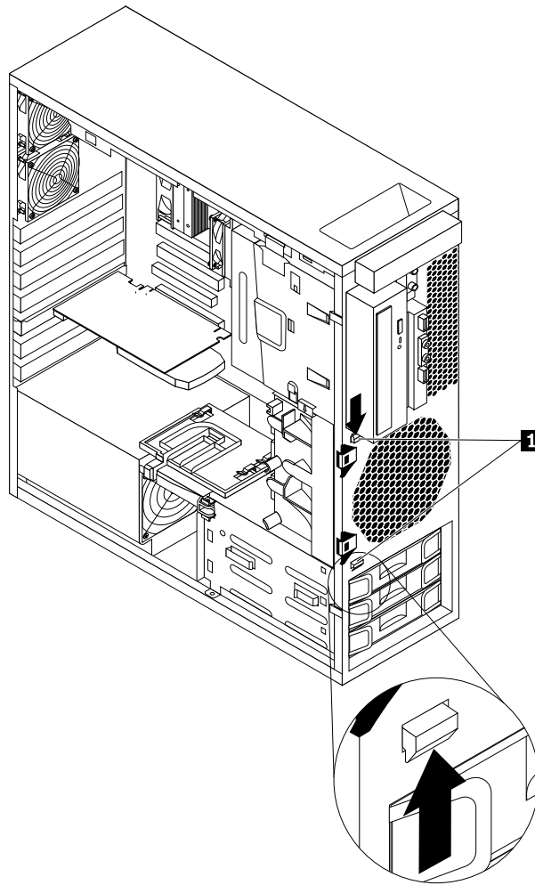
Figure 34. Removing the front fan assembly
