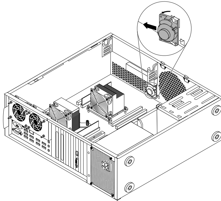
Figure 41. Removing the internal speaker
