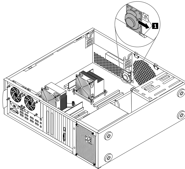
Figure 42. Installing the internal speaker
