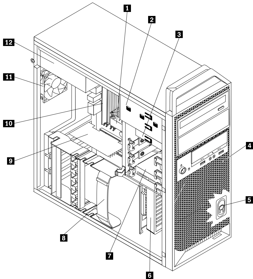
Figure 3. Component locations
