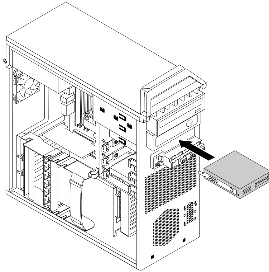
Figure 34. Installing the card reader
