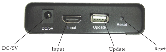
Figure 2: Rear Panel
