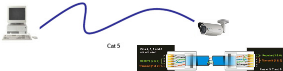
Right: Pinout of a crossed-over cable.
