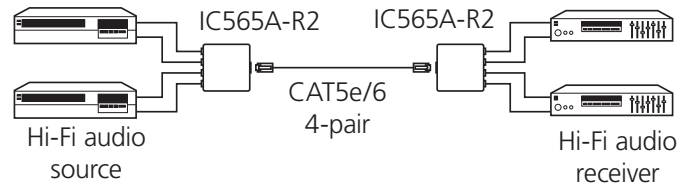
Figure 2. Typical application.
