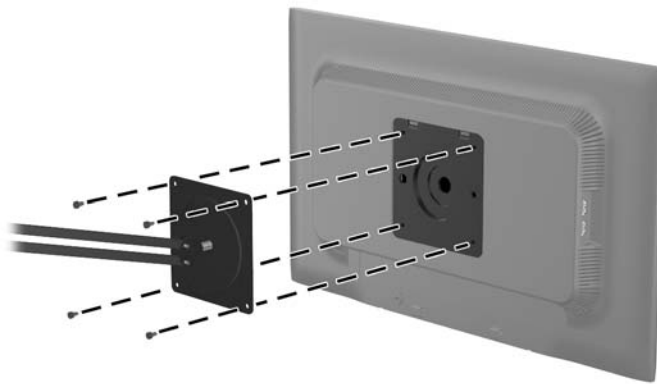
Figure 3-13 Mounting the Monitor
