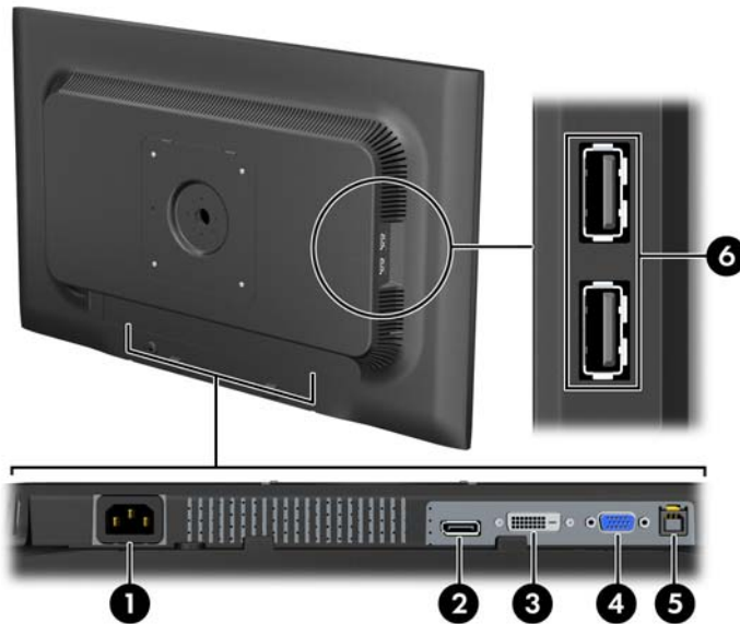
Figure 3-2 Rear Components
