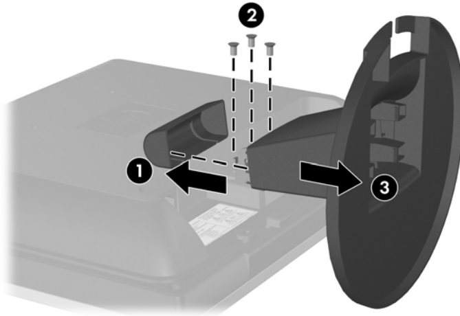
Figure 3-4 Removing the Monitor Pedestal Base
