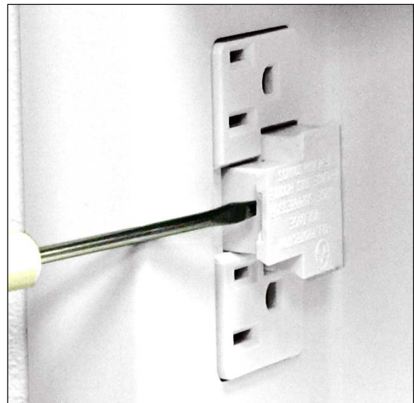
Removing the SurgeBloc® Module
