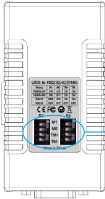
DIP Switches for S1 and S2
