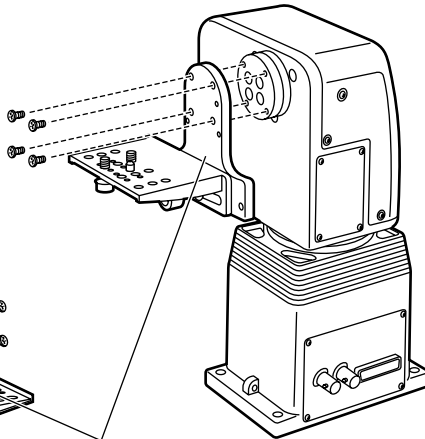
Tilting Arm
