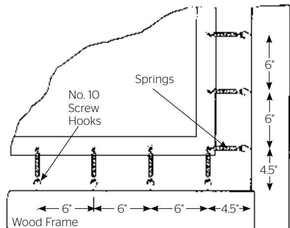
Spring Lacing
