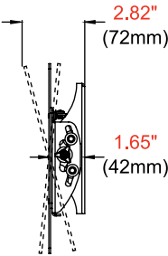
SIDE VIEW VESA 100/200 +15°/-5° TILT
