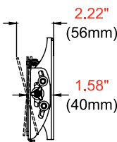
SIDE VIEW VESA 75/100 +15°/-5° TILT
