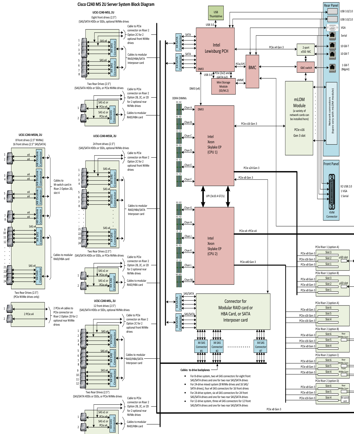
Figure 7 C240 M5 Block Diagram
