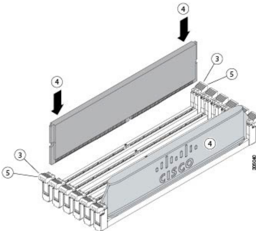
Figure 15 Replacing Memory
