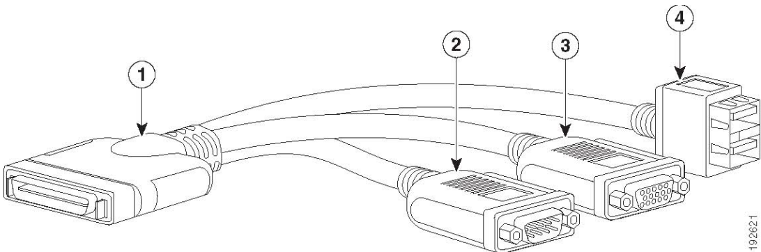
Figure 14 KVM Cable
