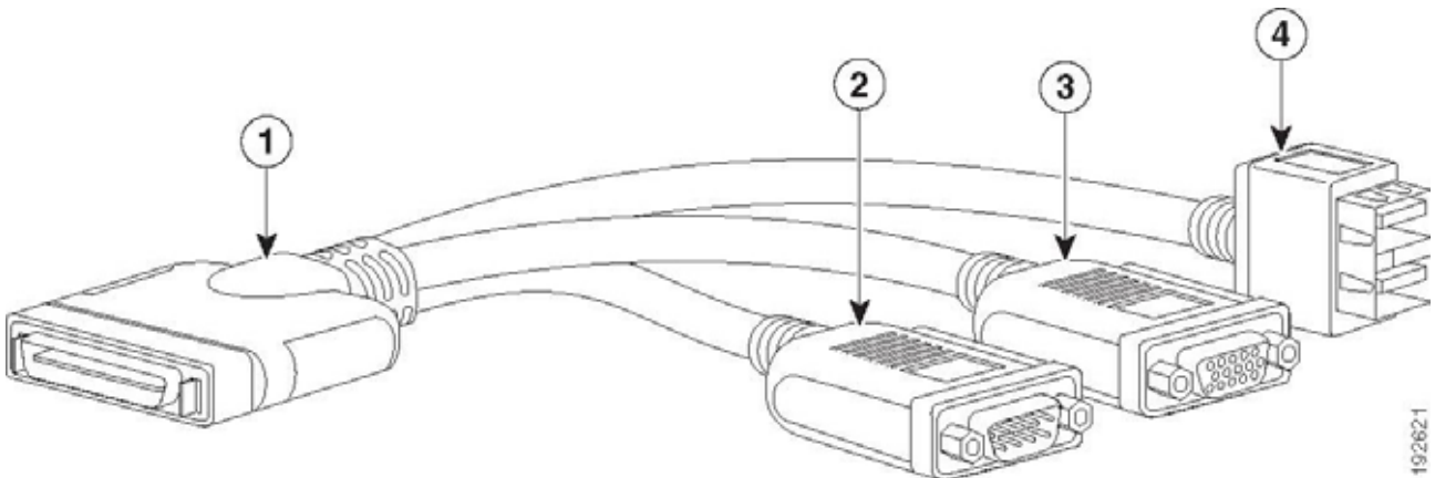
Figure 12 KVM Cable
