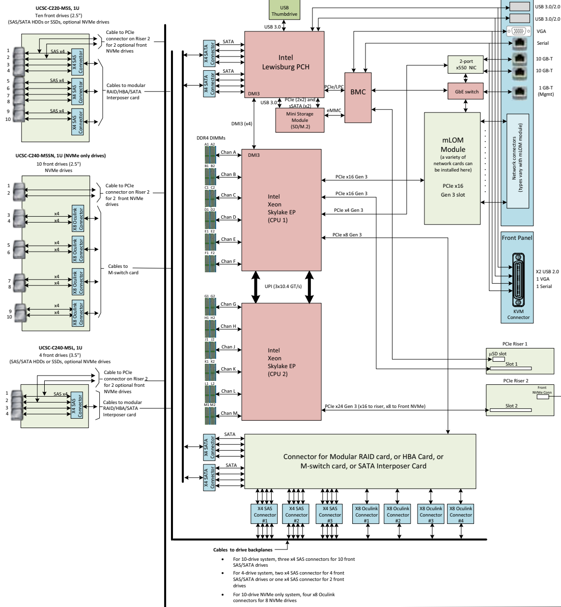
Cisco C240 M5 1U Server System Block Diagram
