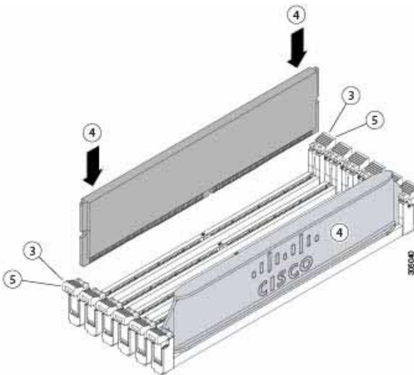
Figure 13 Replacing Memory
