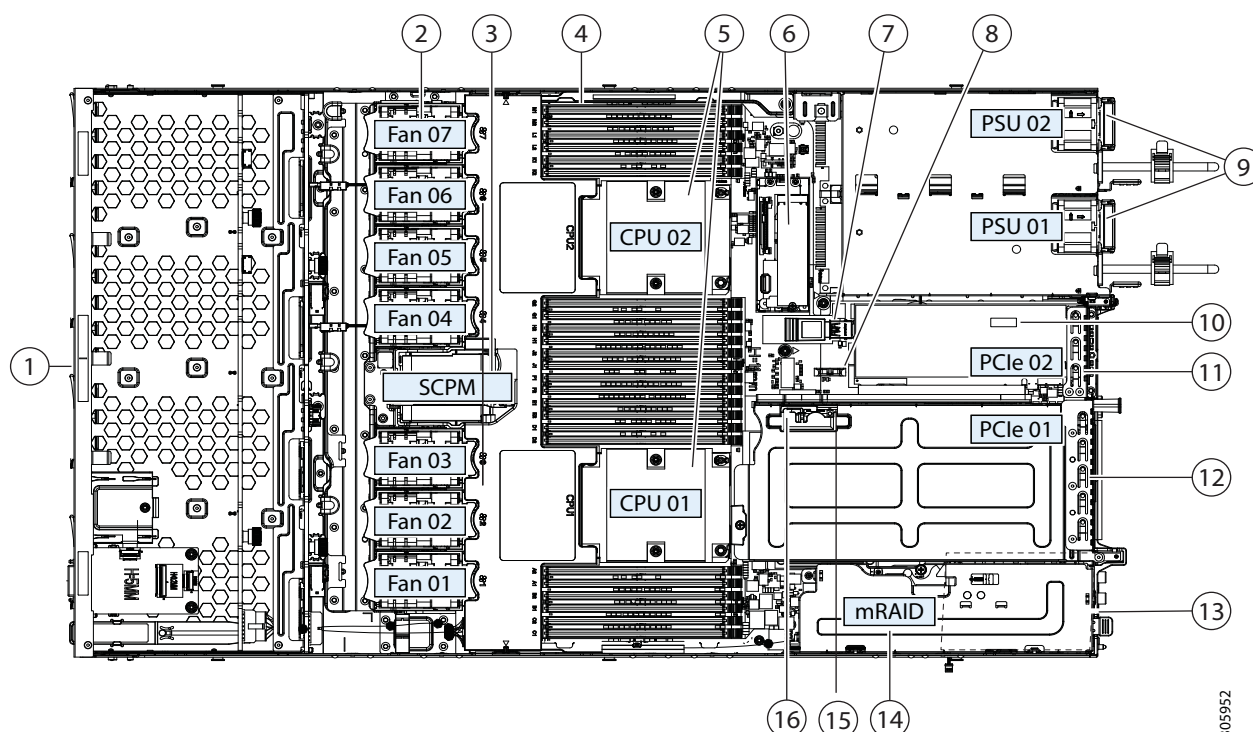
Figure 5 C220 M5 SFF With Top Cover Off
