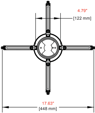
TOP VIEW OF ADAPTER PLATE
