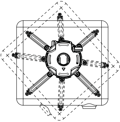
SWIVEL (YAW) 360° (when attached to an extension column), ±15° (when flush mounted)
