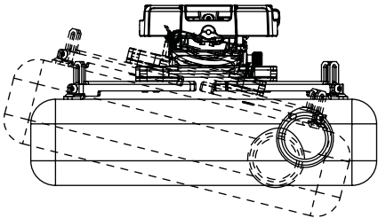
±10° ROLL
