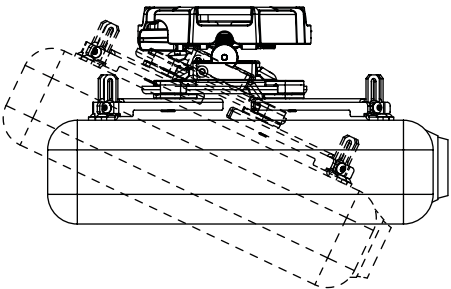
± 20° PITCH
