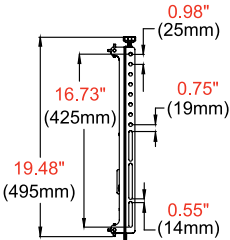
ADAPTOR BRACKET DETAIL
