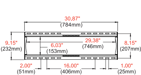
WALL PLATE
