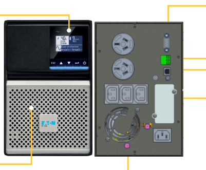
5P Gen2 1550 Tower model
