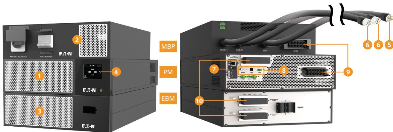
Back of 5 kW UPS (7.5 kW UPS is similar, but with 30A input/output instead of 20A.)
