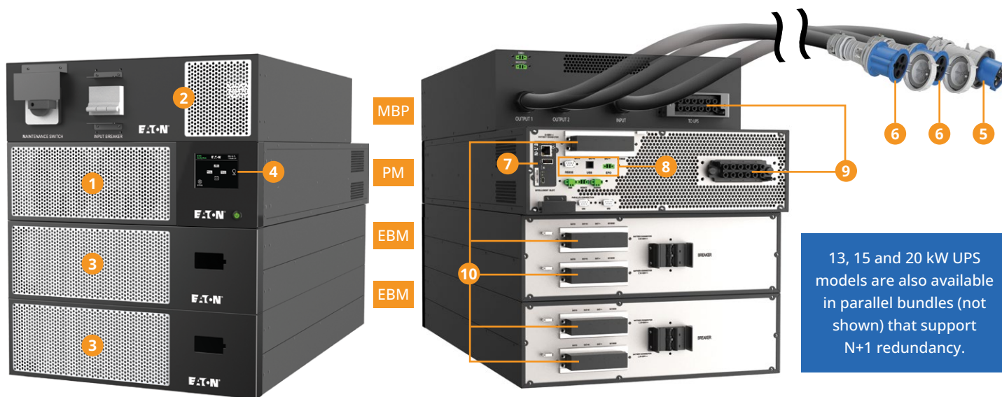
Back of 13 and 15 kW UPS (20 kW UPS is similar, but with hardwired input. Hardwired input and output are also available for 13, 15 and 20 kW UPS systems.)
