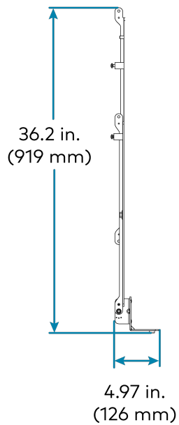
UC-SB2-DMK without the Crestron Videobar
