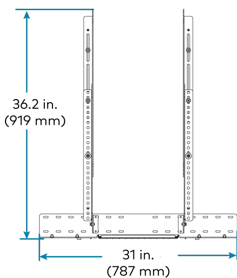
UC-SB2-DMK without the Crestron Videobar
