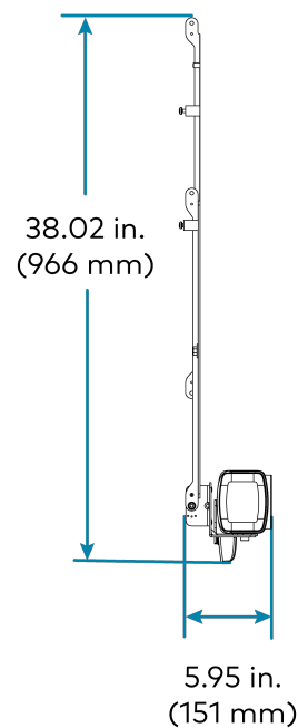
UC-SB2-DMK with the Crestron Videobar
