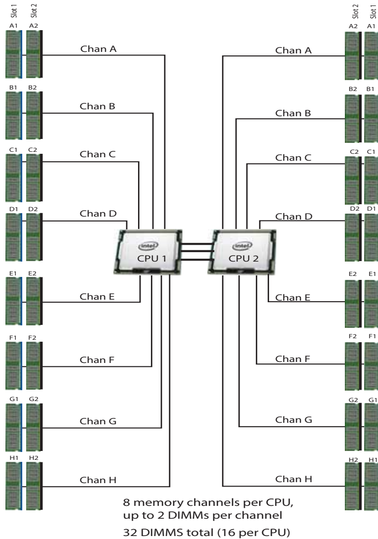
Figure 4 X210c M7 SFF Memory Organization
