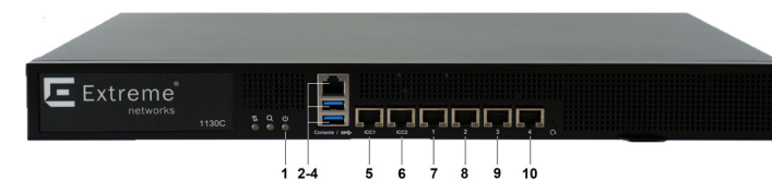
Figure 1: Network Platform 1130C Ports
