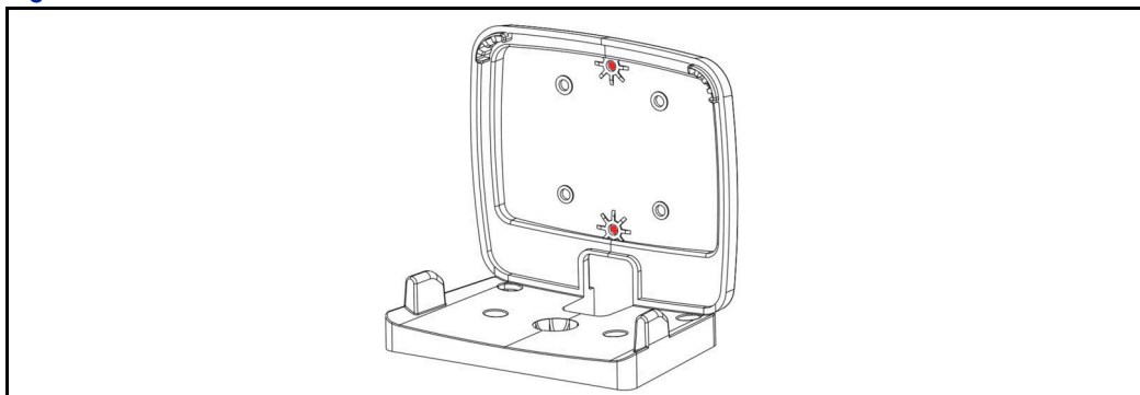
Figure 8. Wall Mount Drill Location
