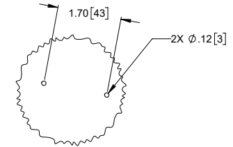
DETAIL A SCALE 1 : 2 6 LOCATIONS
