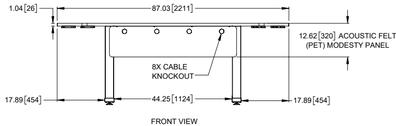
FRONT VIEW WIREMOLD MODPOWER™ ACCESSORIES SEE NOTE 3
