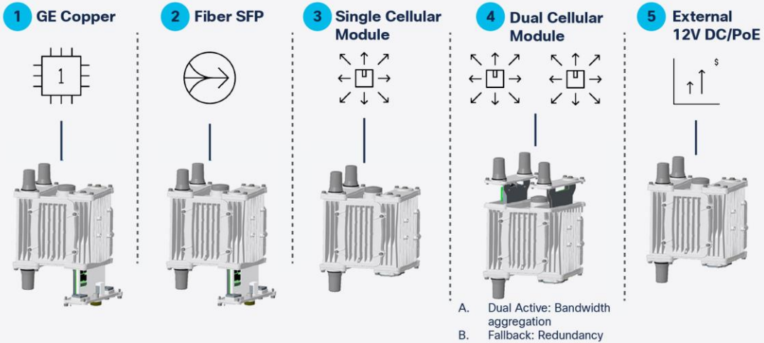
Figure 6. Backhaul options
