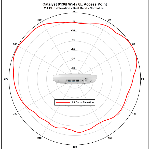
Figure 4: C9136I - Dual-Band Antenna Radiation Pattern (2.4-GHz Elevation)
