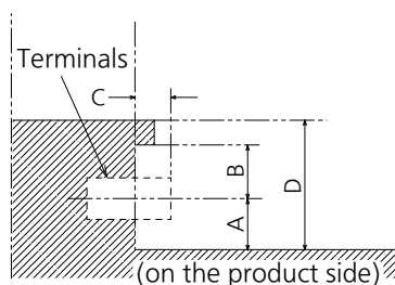
Sectional view of terminal b (AUDIO OUT R / AUDIO OUT L / USB / ANTENNA / CABLE IN / AUDIO IN / PC IN / HDMI 1)
