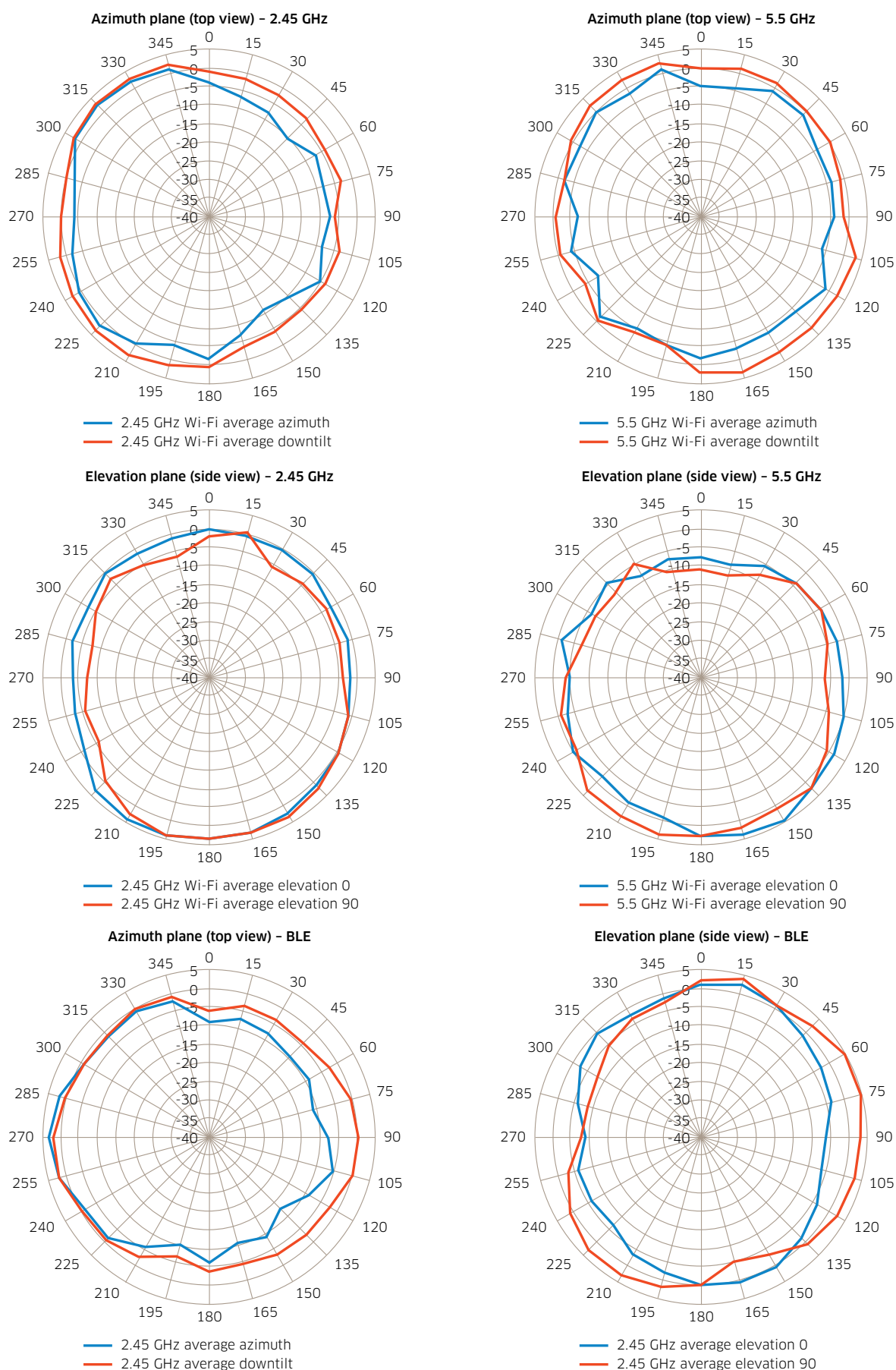
Figures. OmniAccess AP1311 antenna pattern plots
